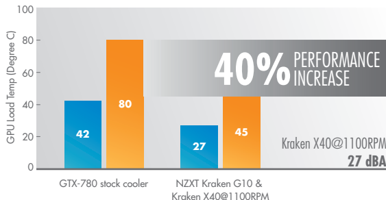
GTX-780 stock cooler vs. NZXT Kraken G10 & Kraken X40 Min Max
